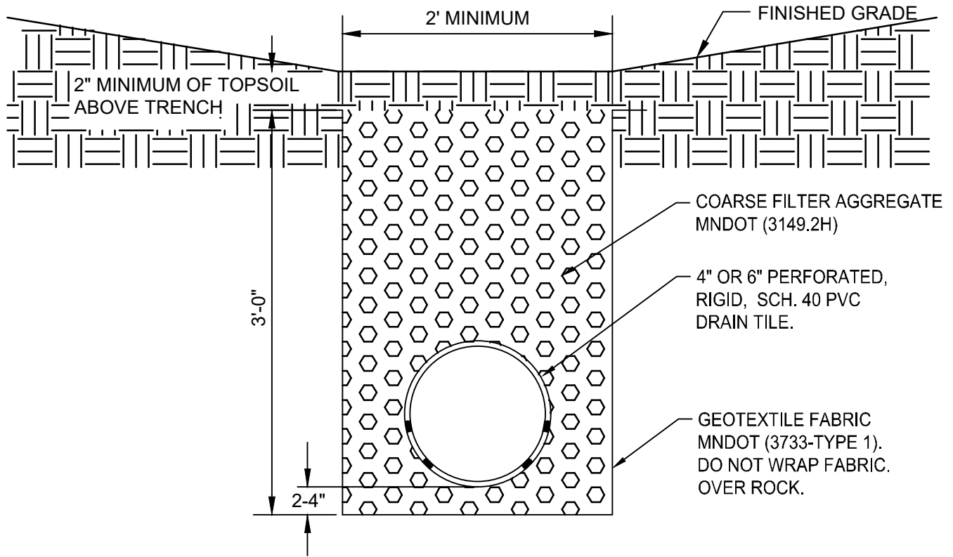
TRENCH DETAIL
