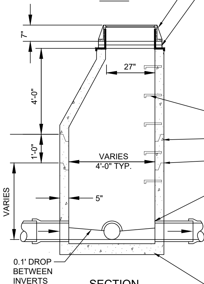
SECTION
