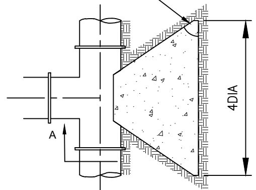
PLAN 3 WAY TEES
