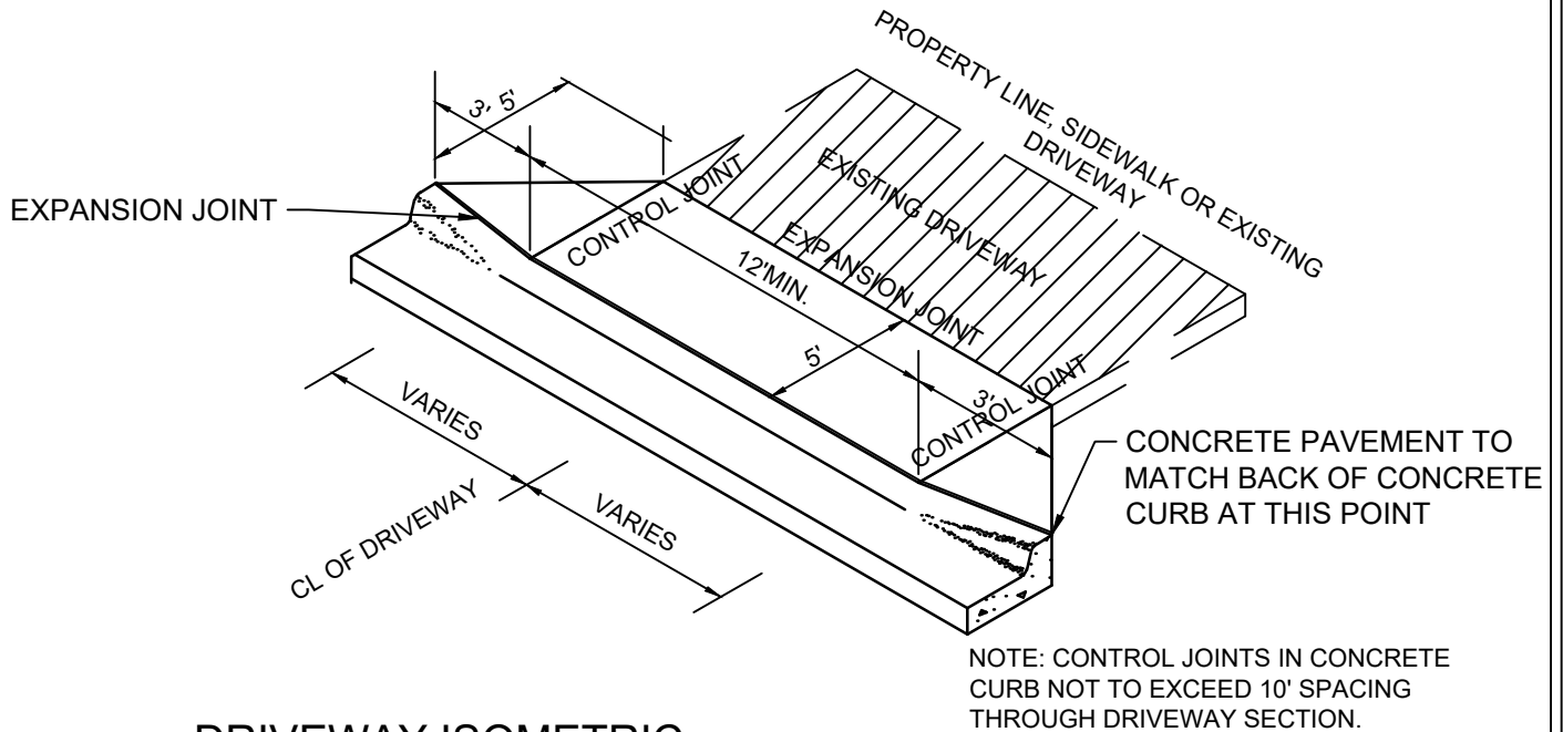
DRIVEWAY ISOMETRIC NO SCALE
