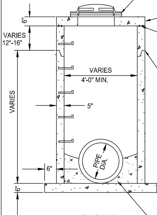
SECTION
